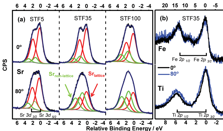
Fig. 2 (a) Comparison of the Sr 3d spectra on STF5, STF35 and STF100 at emission angles of 0^\circ and 80^\circ . The red doublets correspond to the bulk-coordinated \text{Sr}_{\text{lattice}} and the green doublets are attributed to the binding environment on the surface \text{Sr}_{\text{non-lattice}} . The binding energy of the Sr spectra was referenced to the peak position of the 3d_{5/2} peak in the main doublet ( \text{Sr}_{\text{lattice}} ) for comparison. (b) Comparison of the Fe 2p and Ti 2p spectra of STF35 at emission angles of 0^\circ and 80^\circ . The binding energies on the Fe spectra and Ti spectra were referenced to \text{Fe } 2p_{3/2} and \text{Ti } 2p_{3/2} , respectively.
